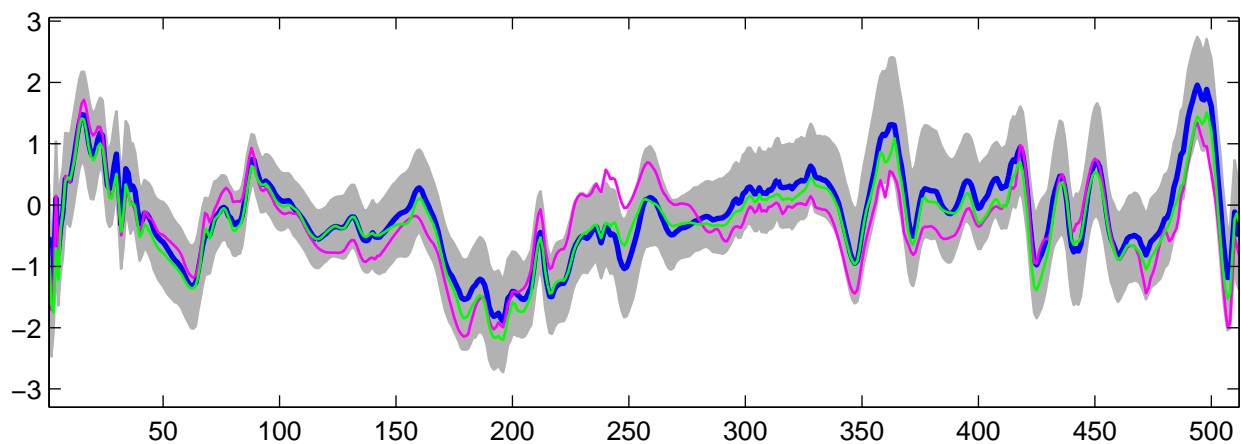
Estimated U_{30}(t) using R-WFMM: Normal data, run 2
