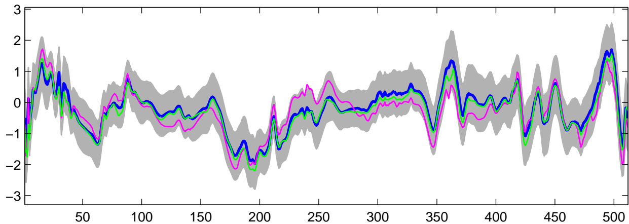
Estimated U_{30}(t) using G-WFMM: Normal data, run 2
