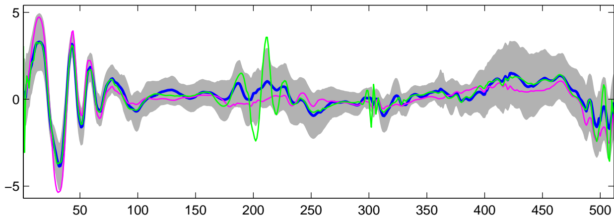
Estimated U_{30}(t) using G-WFMM: t_1 data, run 2
