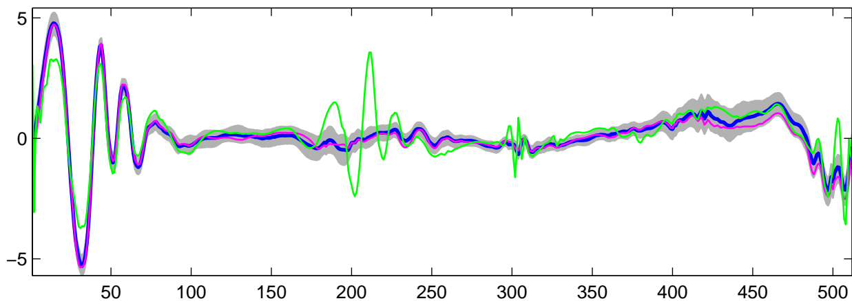
Estimated U_{30}(t) using R-WFMM: t_1 data, run 2
