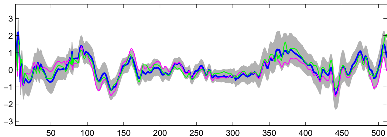
Estimated U_{30}(t) using R-WFMM: t_2 data, run 2
