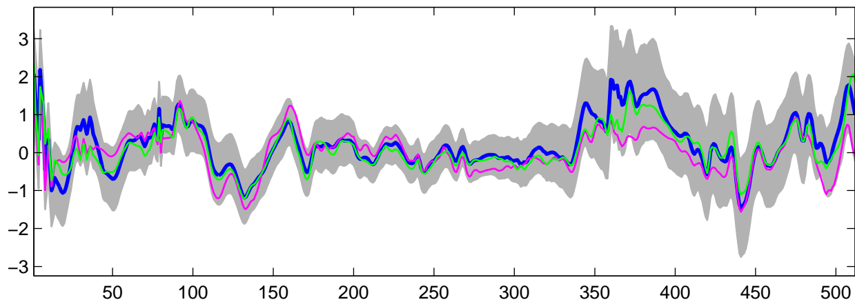
Estimated U_{30}(t) using G-WFMM: t_2 data, run 2
