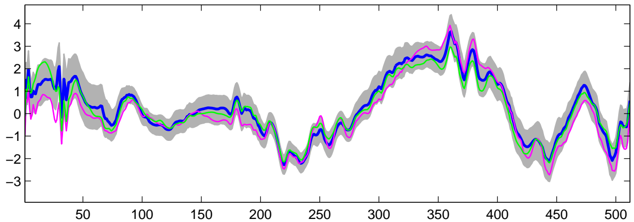
Estimated U_{31}(t) using R-WFMM: DE data, run 2
