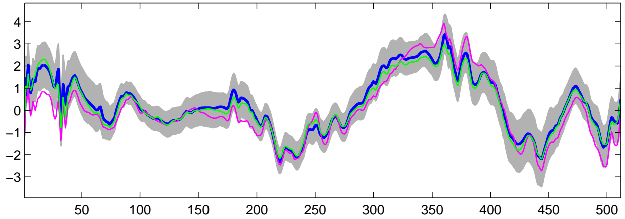
Estimated U_{31}(t) using G-WFMM: DE data, run 2
