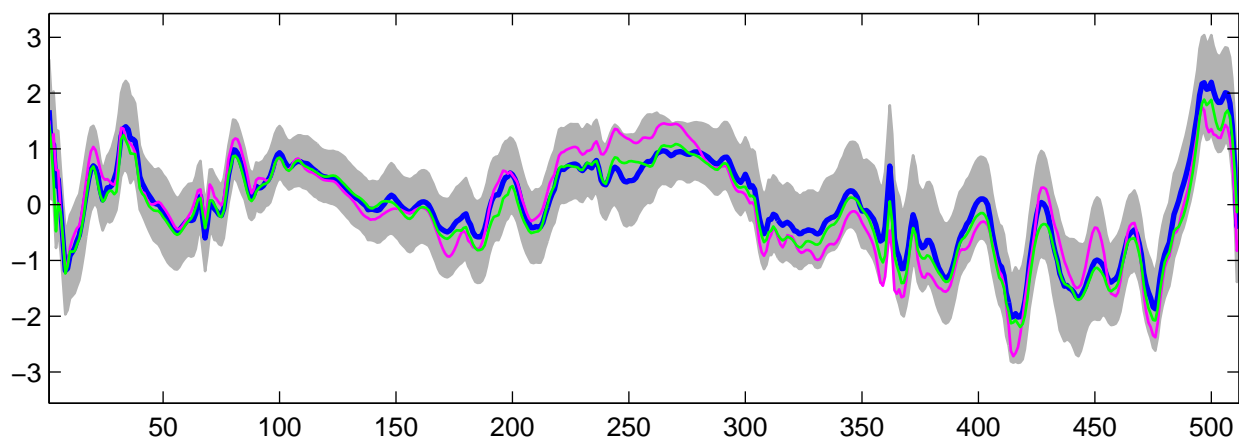
Estimated U_{31}(t) using R-WFMM: Normal data, run 2
