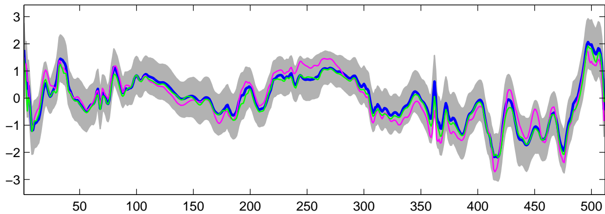
Estimated U_{31}(t) using G-WFMM: Normal data, run 2
