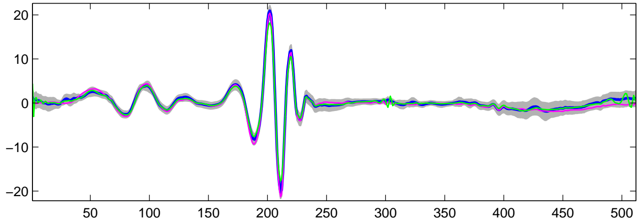
Estimated U_{31}(t) using G-WFMM: t_1 data, run 2
