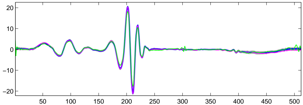
Estimated U_{31}(t) using R-WFMM: t_1 data, run 2
