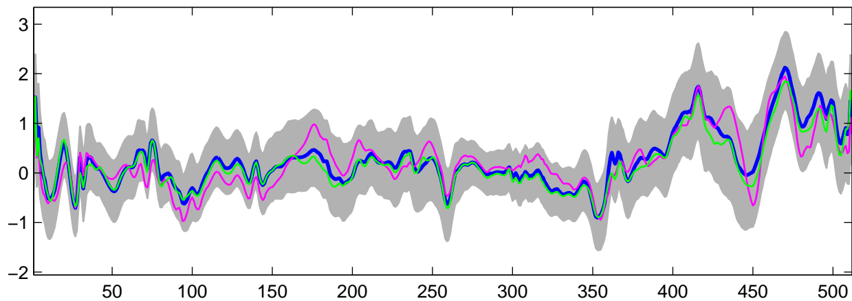
Estimated U_{31}(t) using G-WFMM: t_3 data, run 2
