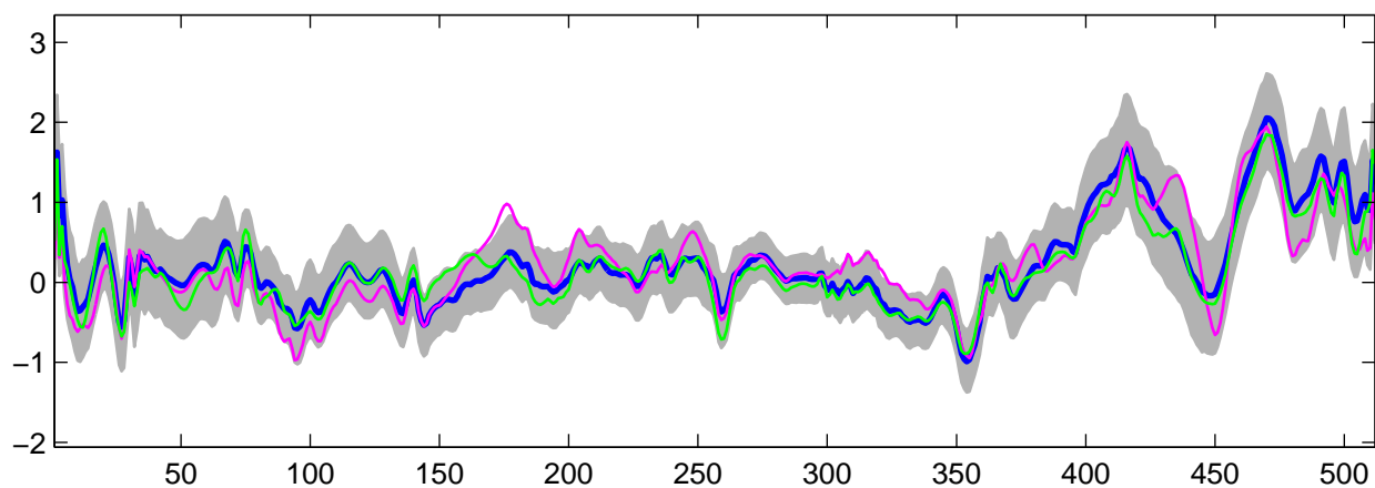
Estimated U_{31}(t) using R-WFMM: t_3 data, run 2
