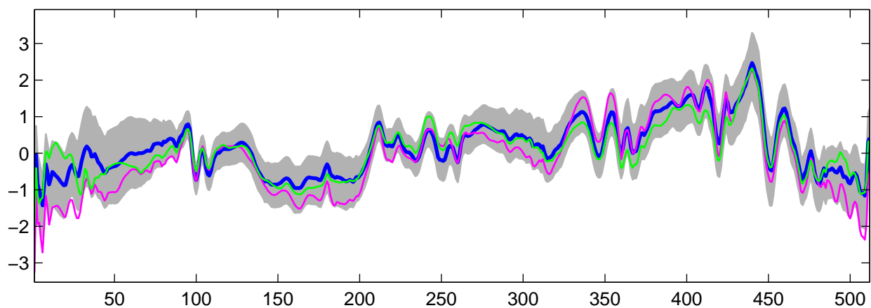
Estimated U_{32}(t) using R-WFMM: DE data, run 2
