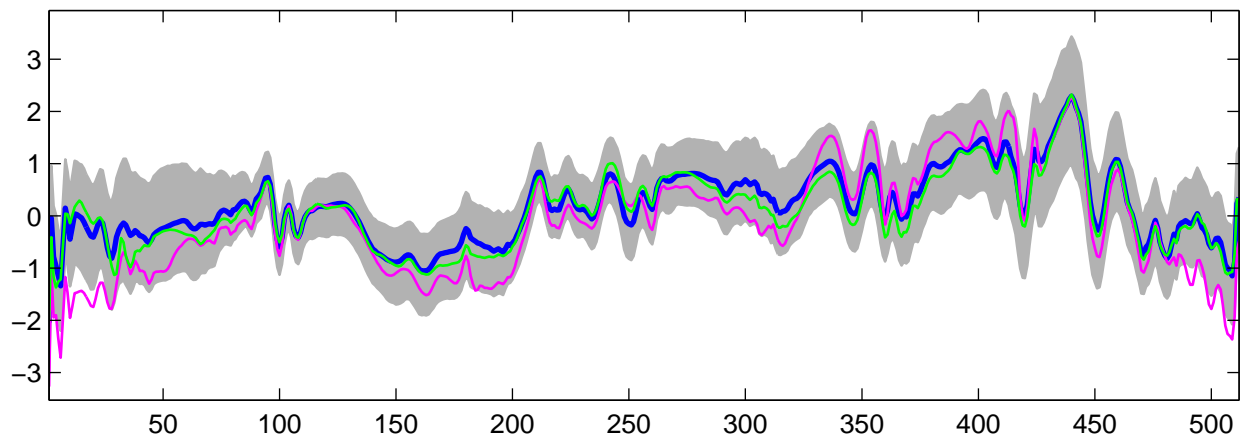
Estimated U_{32}(t) using G-WFMM: DE data, run 2
