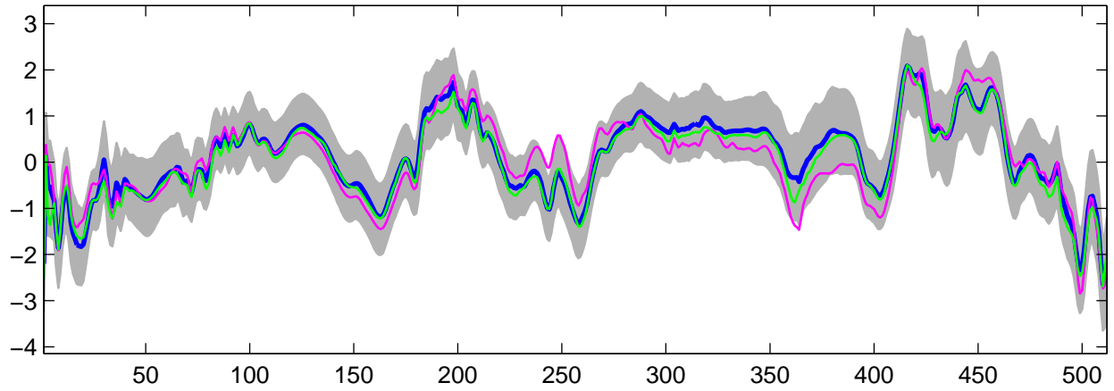
Estimated U_{32}(t) using G-WFMM: Normal data, run 2
