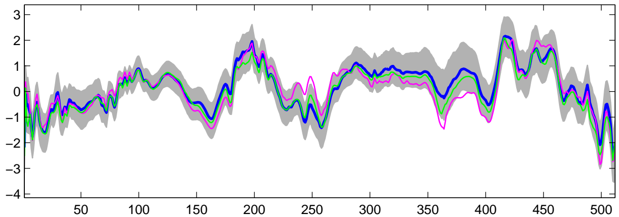
Estimated U_{32}(t) using R-WFMM: Normal data, run 2
