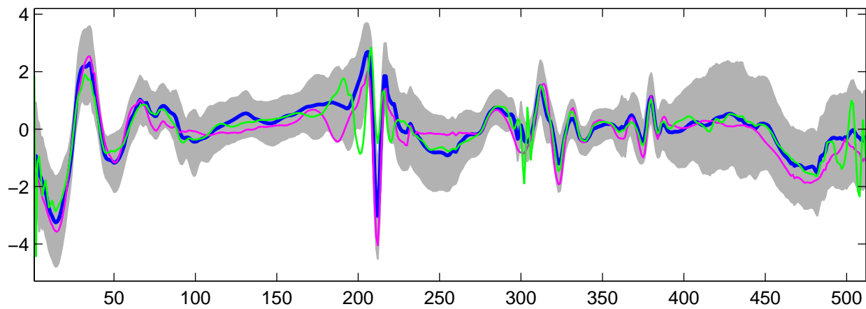
Estimated U_{32}(t) using G-WFMM: t_1 data, run 2
