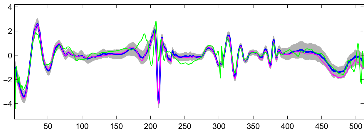
Estimated U_{32}(t) using R-WFMM: t_1 data, run 2
