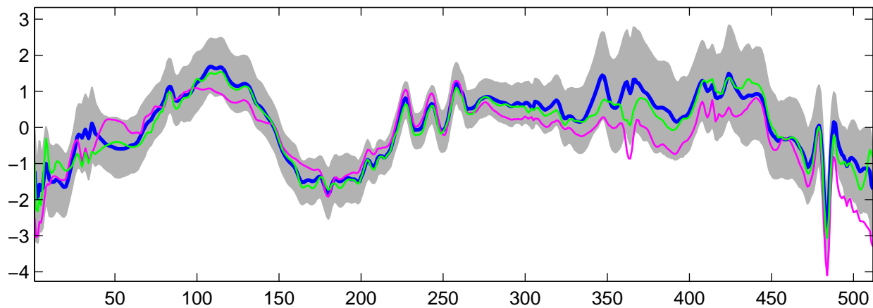
Estimated U_{32}(t) using G-WFMM: t_2 data, run 2
