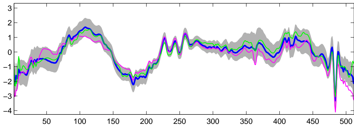
Estimated U_{32}(t) using R-WFMM: t_2 data, run 2
