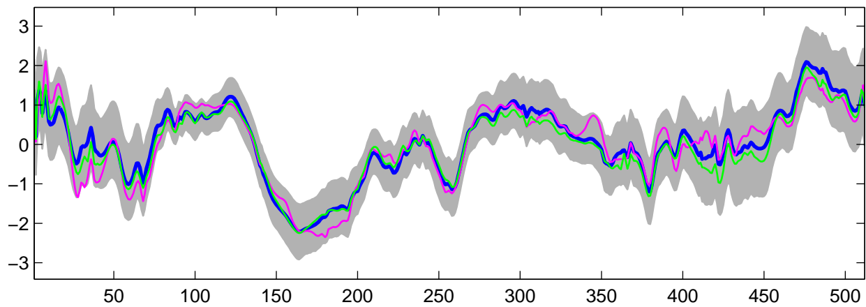
Estimated U_3(t) using G-WFMM: DE data, run 2
