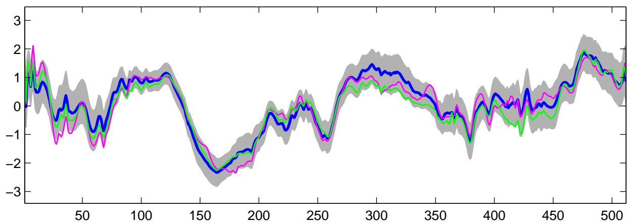
Estimated U_3(t) using R-WFMM: DE data, run 2
