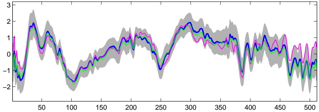
Estimated U_3(t) using G-WFMM: Normal data, run 2
