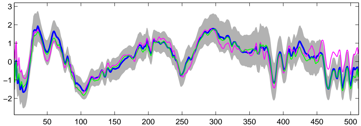
Estimated U_3(t) using R-WFMM: Normal data, run 2
