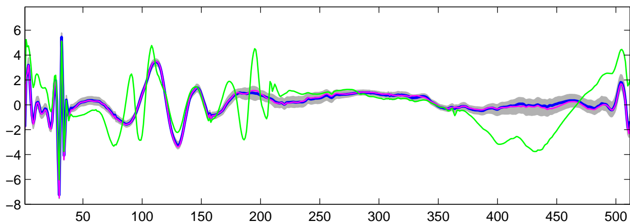
Estimated U_3(t) using R-WFMM: t_1 data, run 2
