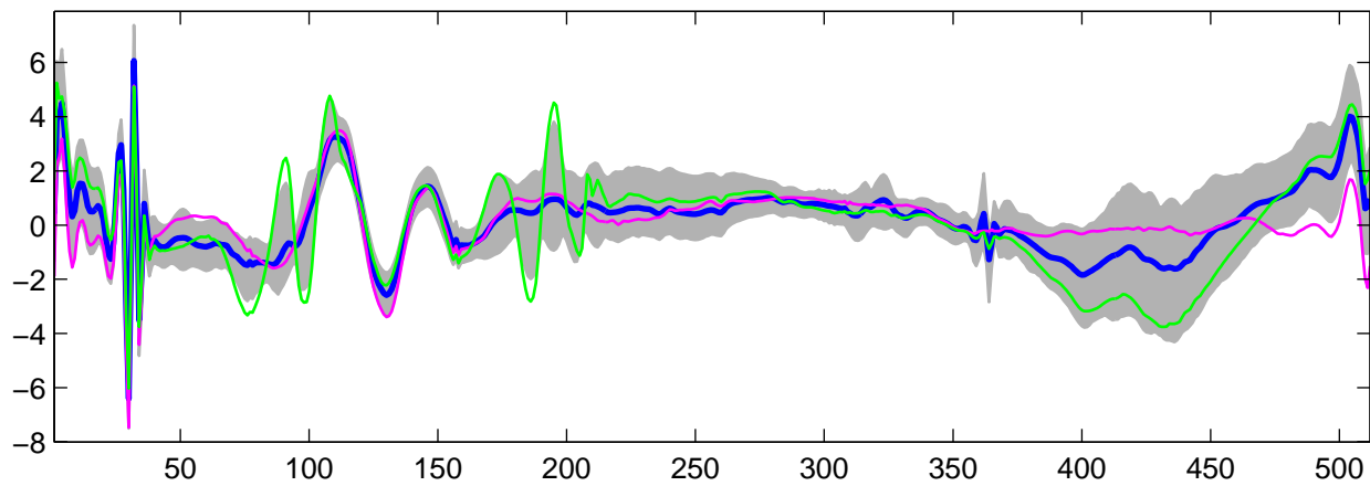
Estimated U_3(t) using G-WFMM: t_1 data, run 2
