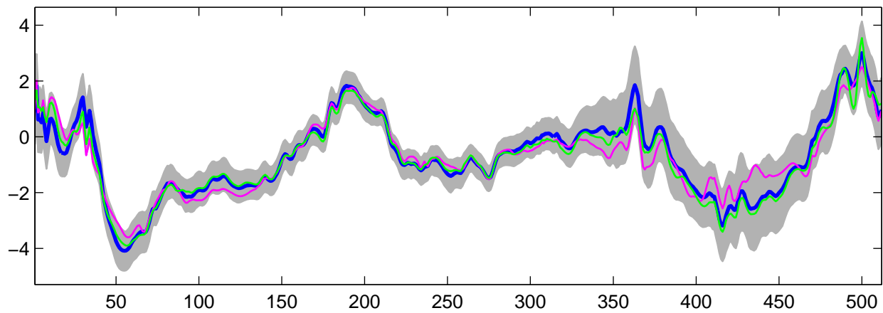
Estimated U_3(t) using G-WFMM: t_2 data, run 2
