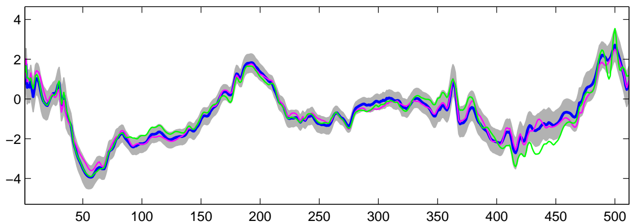
Estimated U_3(t) using R-WFMM: t_2 data, run 2
