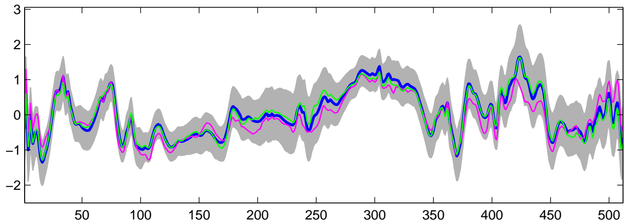
Estimated U_3(t) using G-WFMM: t_3 data, run 2
