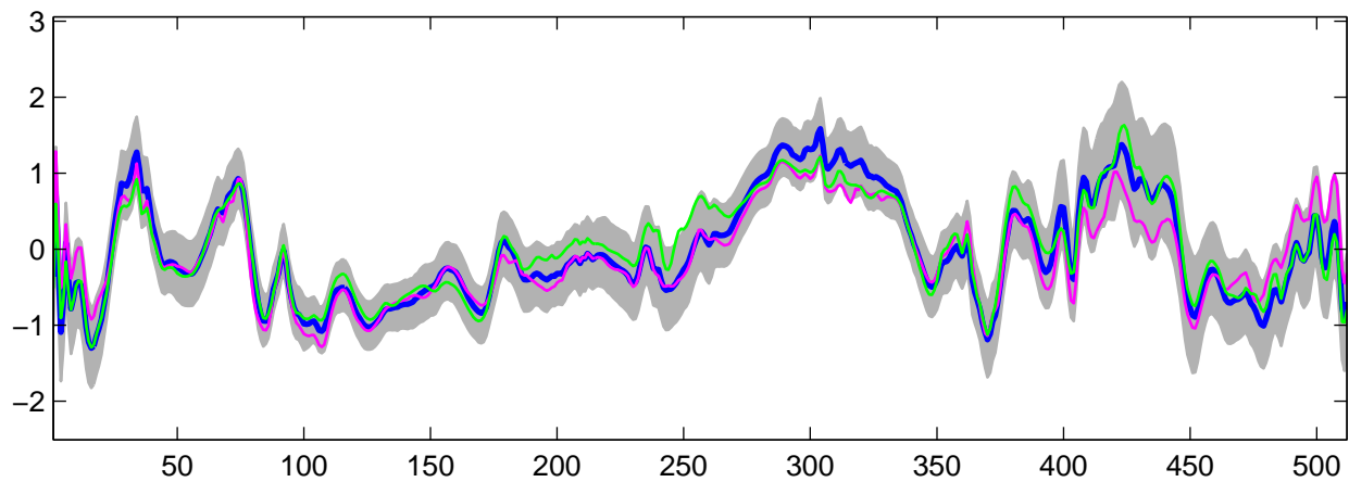
Estimated U_3(t) using R-WFMM: t_3 data, run 2
