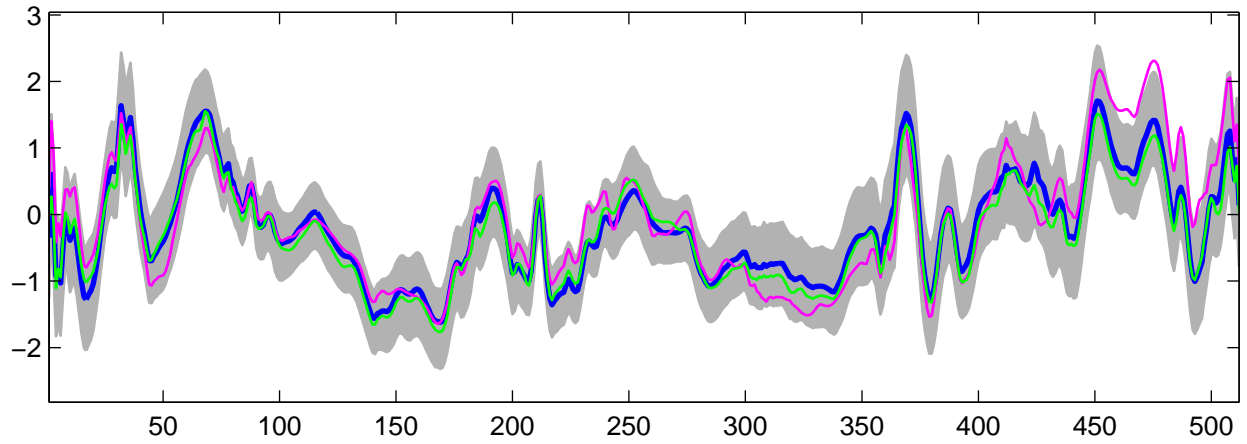
Estimated U_4(t) using G-WFMM: Normal data, run 2
