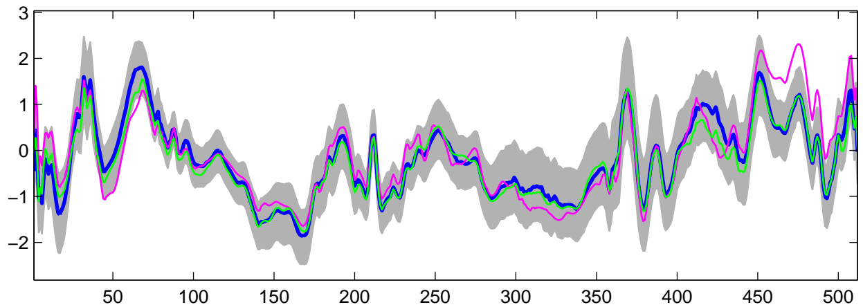
Estimated U_4(t) using R-WFMM: Normal data, run 2
