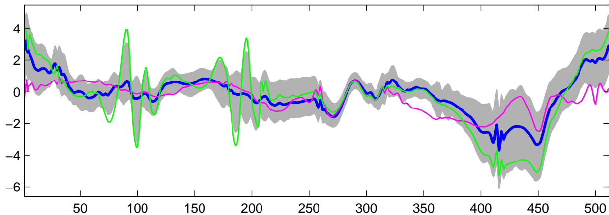
Estimated U_4(t) using G-WFMM: t_1 data, run 2
