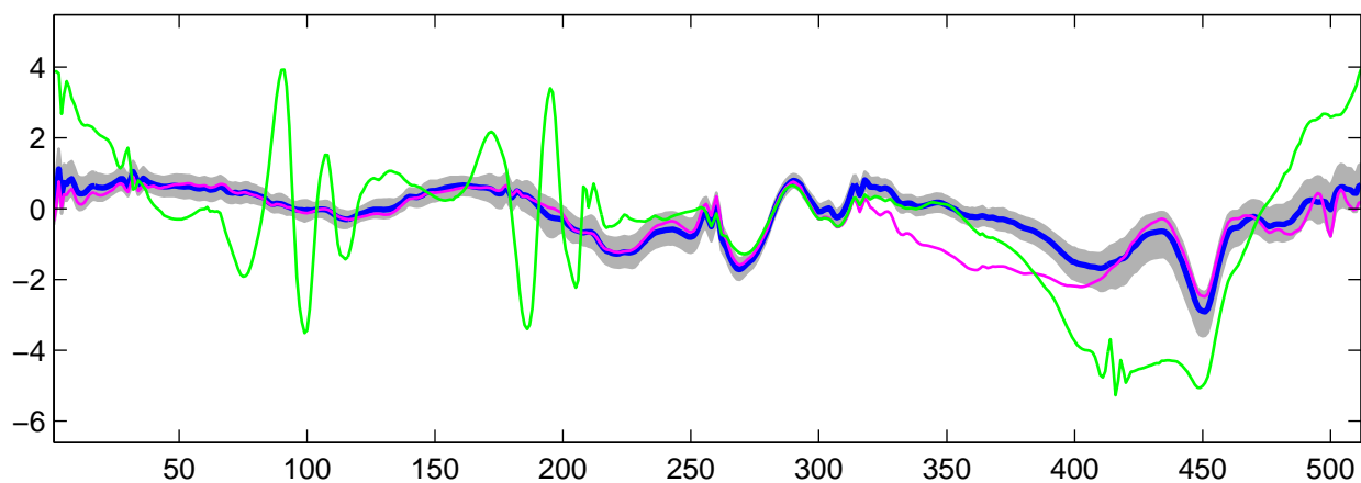
Estimated U_4(t) using R-WFMM: t_1 data, run 2
