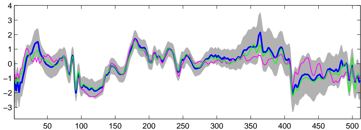
Estimated U_4(t) using G-WFMM: t_2 data, run 2
