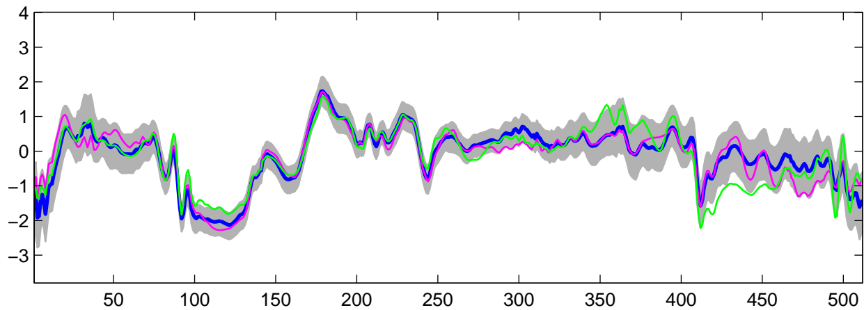
Estimated U_4(t) using R-WFMM: t_2 data, run 2
