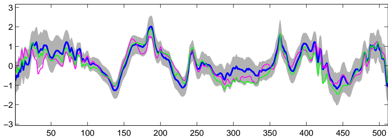
Estimated U_5(t) using R-WFMM: DE data, run 2
