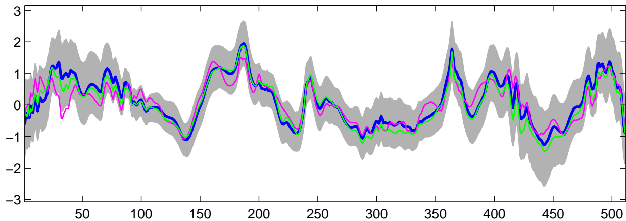
Estimated U_5(t) using G-WFMM: DE data, run 2
