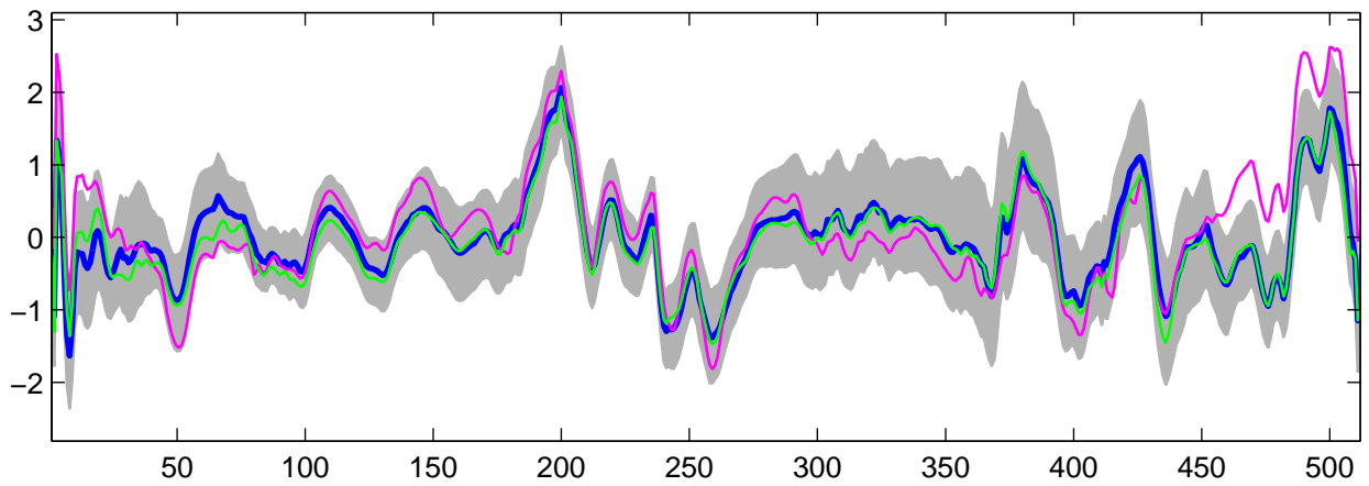
Estimated U_5(t) using R-WFMM: Normal data, run 2
