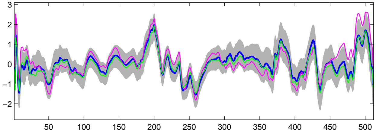
Estimated U_5(t) using G-WFMM: Normal data, run 2
