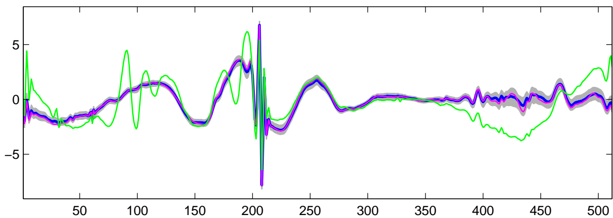
Estimated U_5(t) using R-WFMM: t_1 data, run 2
