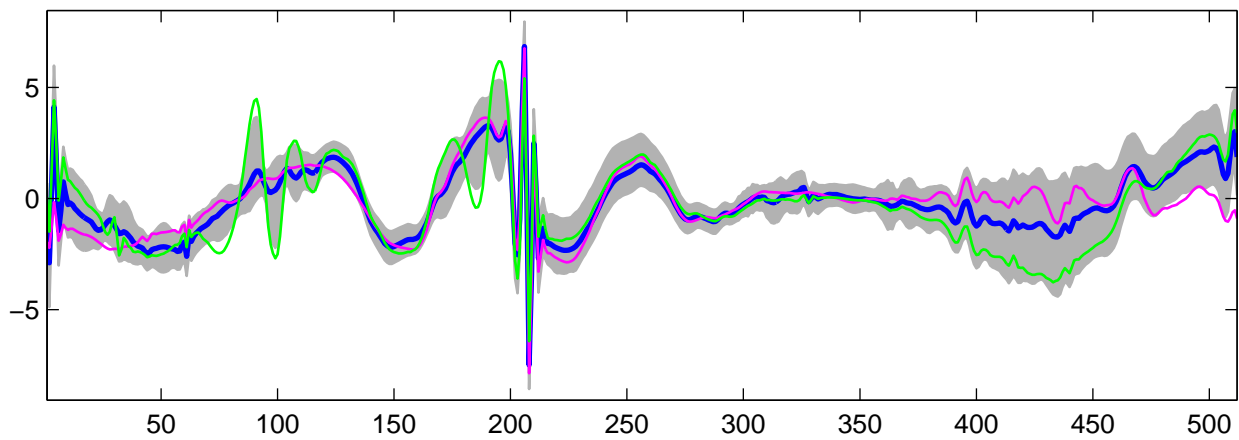
Estimated U_5(t) using G-WFMM: t_1 data, run 2
