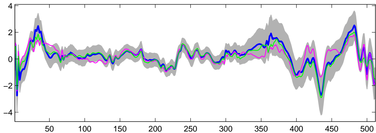
Estimated U_5(t) using G-WFMM: t_2 data, run 2
