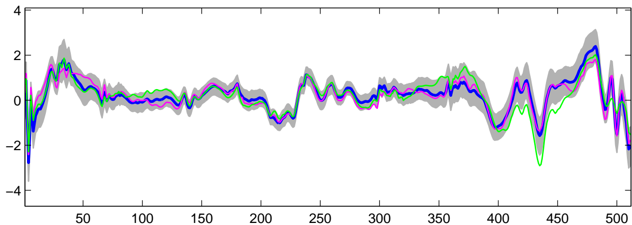
Estimated U_5(t) using R-WFMM: t_2 data, run 2
