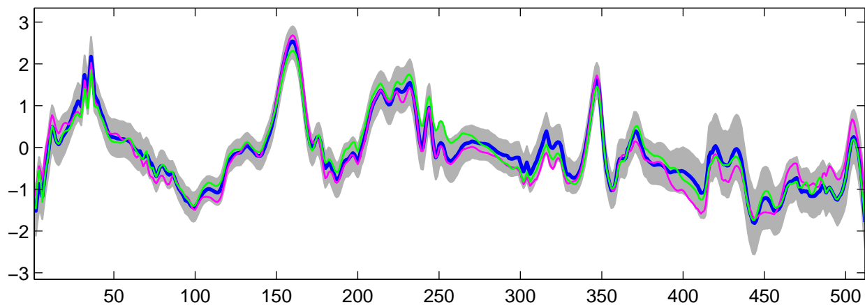
Estimated U_5(t) using R-WFMM: t_3 data, run 2
