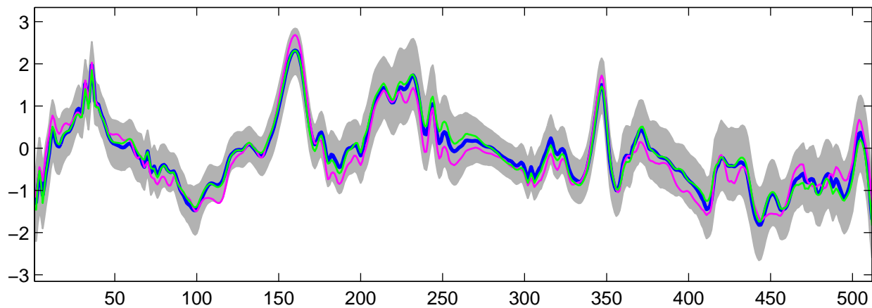
Estimated U_5(t) using G-WFMM: t_3 data, run 2
