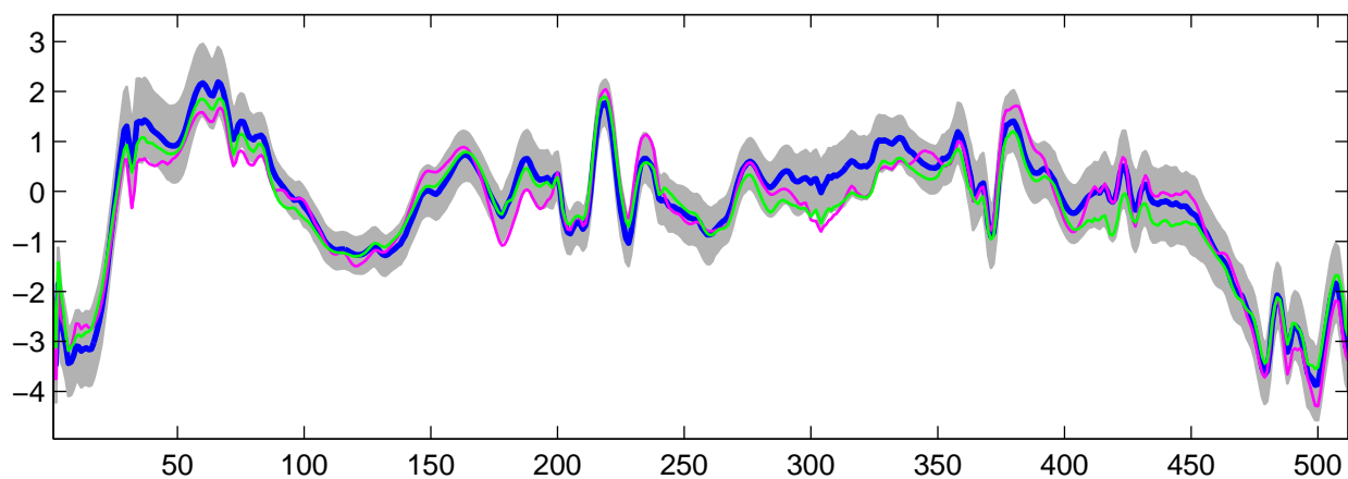
Estimated U_6(t) using R-WFMM: DE data, run 2
