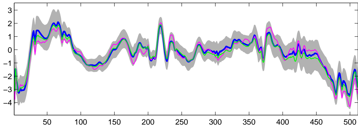
Estimated U_6(t) using G-WFMM: DE data, run 2
