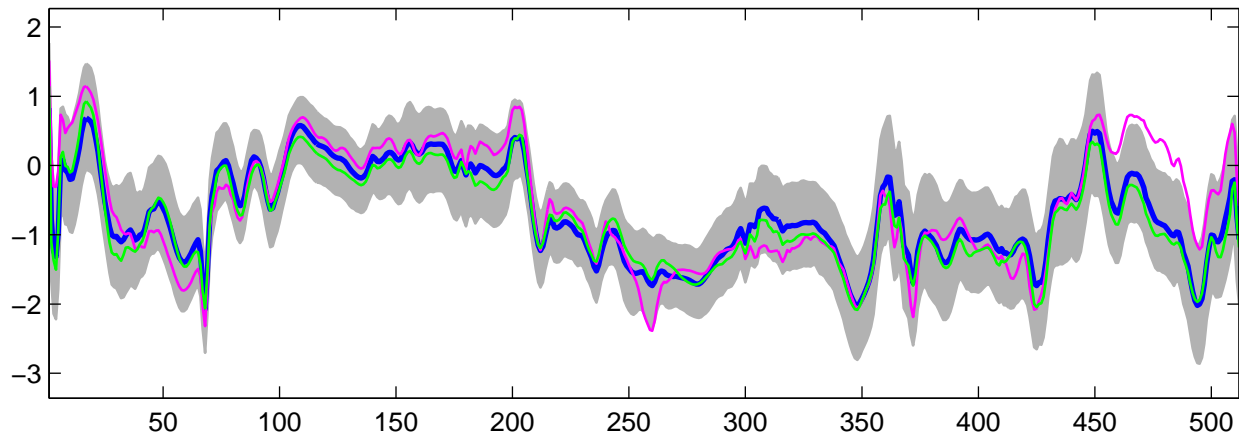
Estimated U_6(t) using G-WFMM: Normal data, run 2
