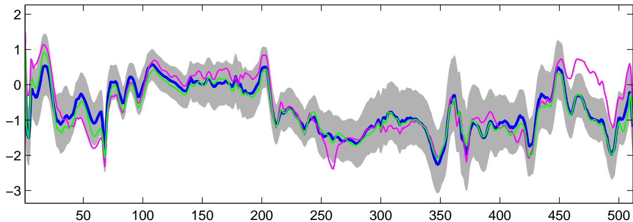
Estimated U_6(t) using R-WFMM: Normal data, run 2
