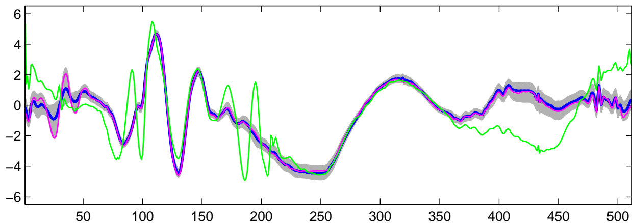
Estimated U_6(t) using R-WFMM: t_1 data, run 2
