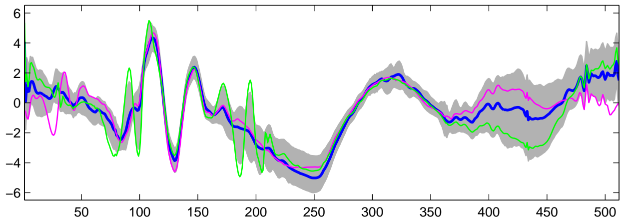
Estimated U_6(t) using G-WFMM: t_1 data, run 2
