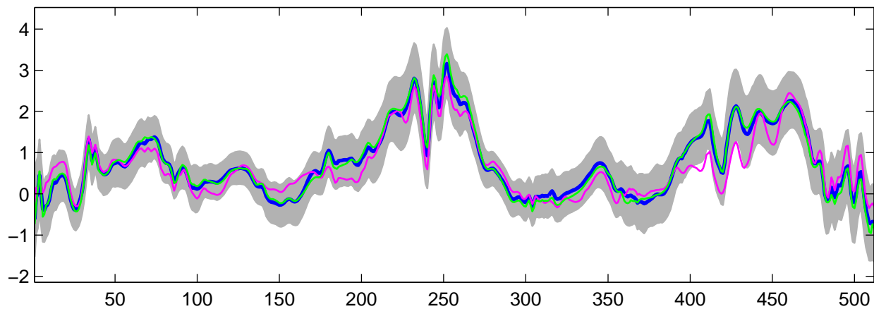
Estimated U_6(t) using G-WFMM: t_3 data, run 2
