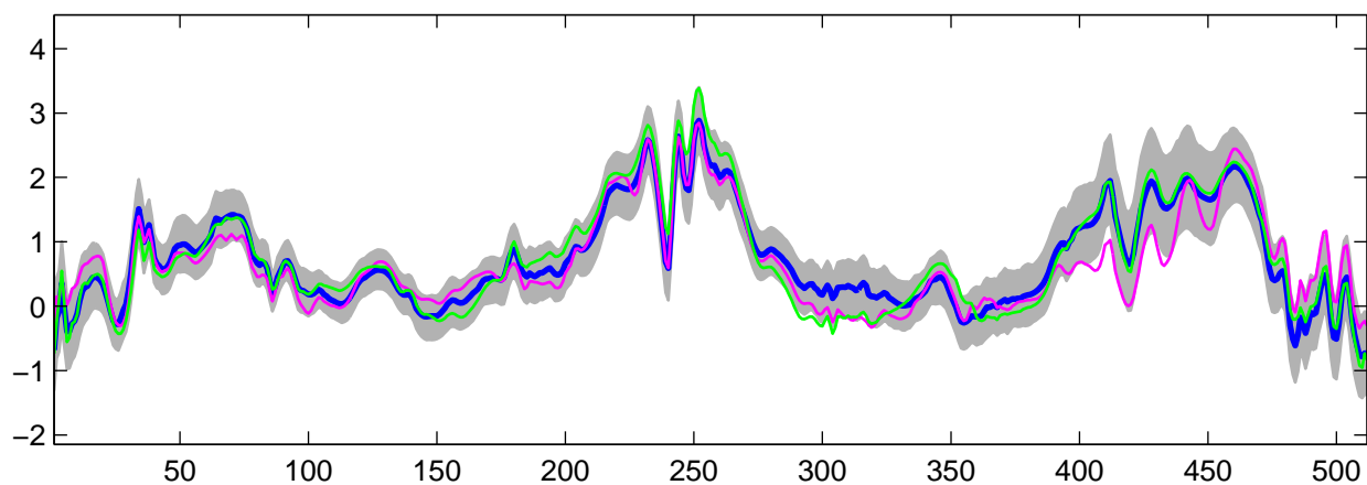
Estimated U_6(t) using R-WFMM: t_3 data, run 2
