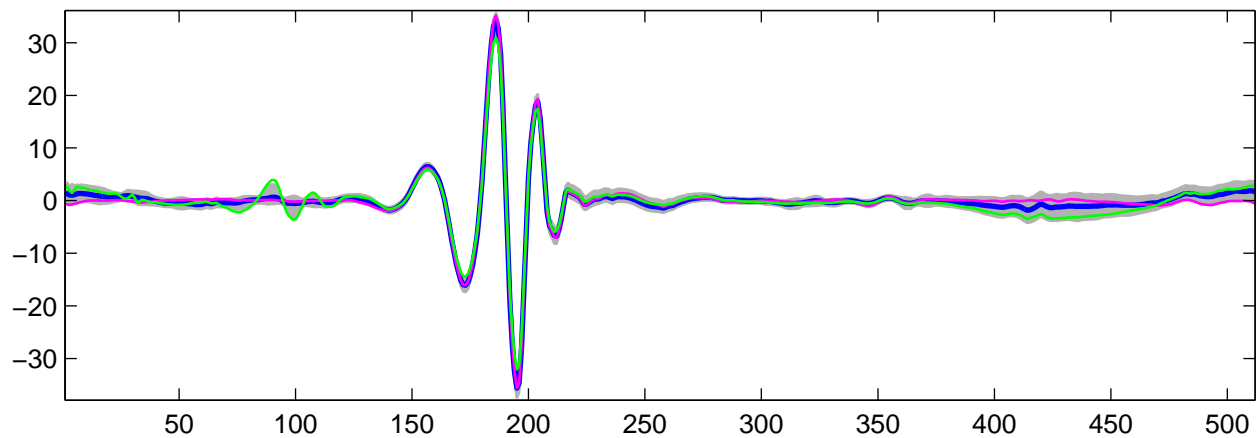
Estimated U_7(t) using G-WFMM: t_1 data, run 2
