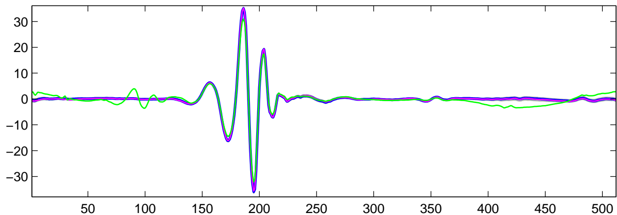
Estimated U_7(t) using R-WFMM: t_1 data, run 2
