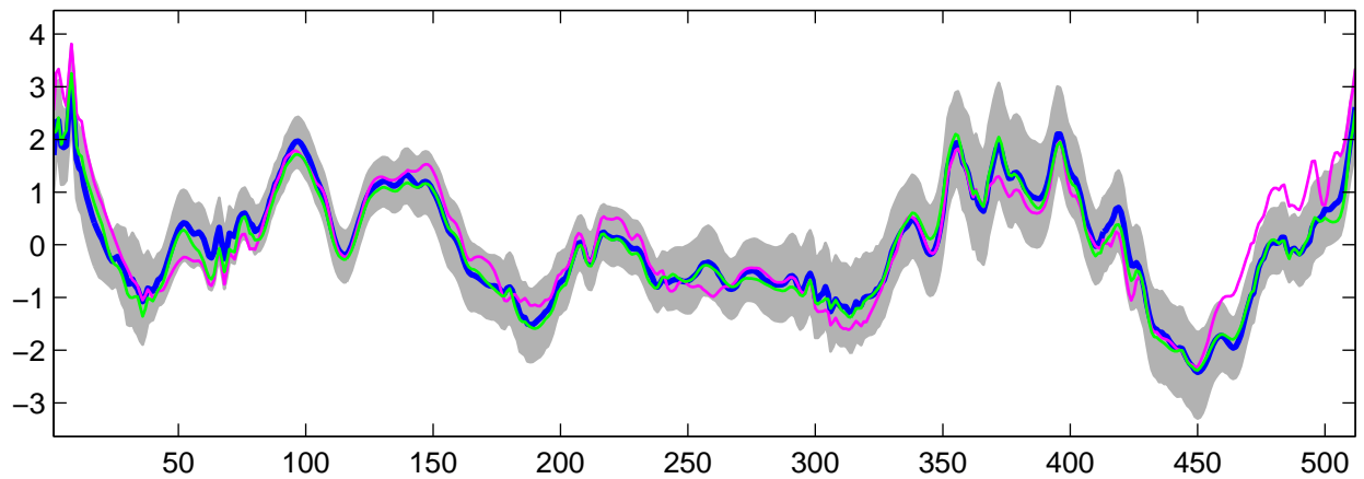
Estimated U_g(t) using R-WFMM: Normal data, run 2
