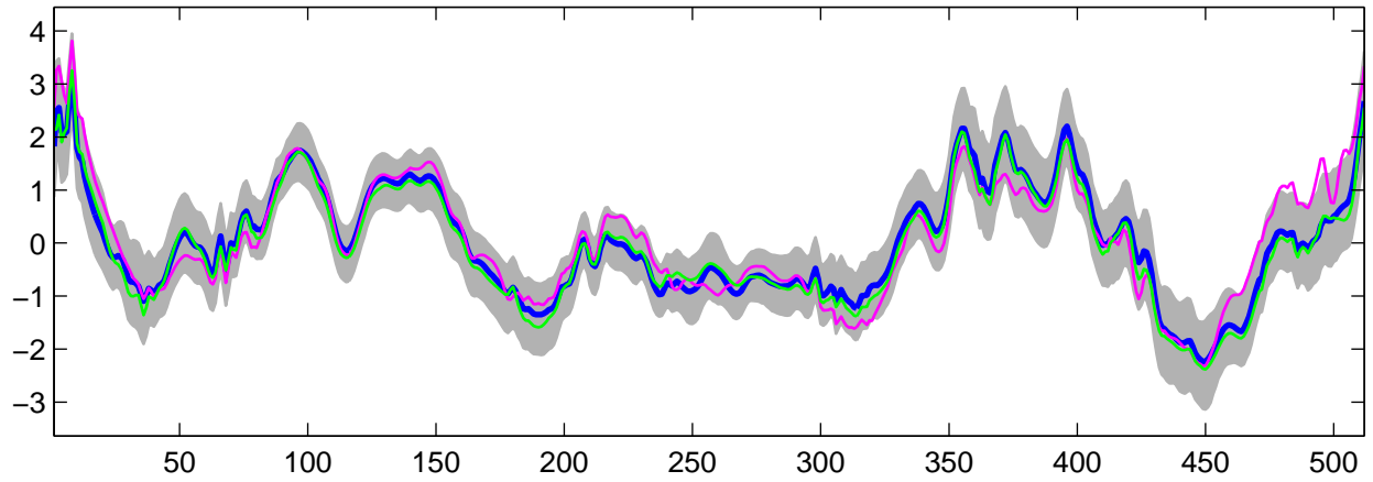
Estimated U_g(t) using G-WFMM: Normal data, run 2
