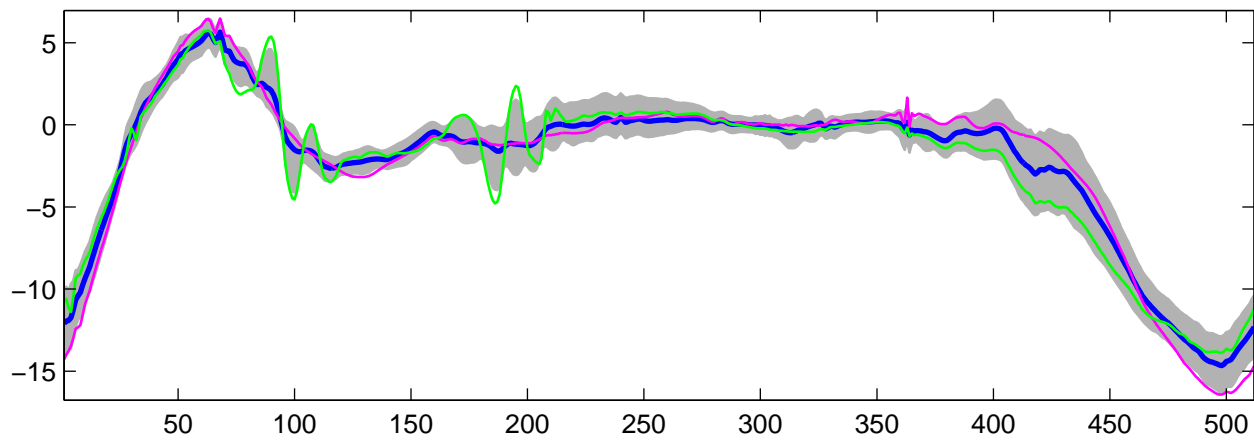
Estimated U_8(t) using G-WFMM: t_1 data, run 2
