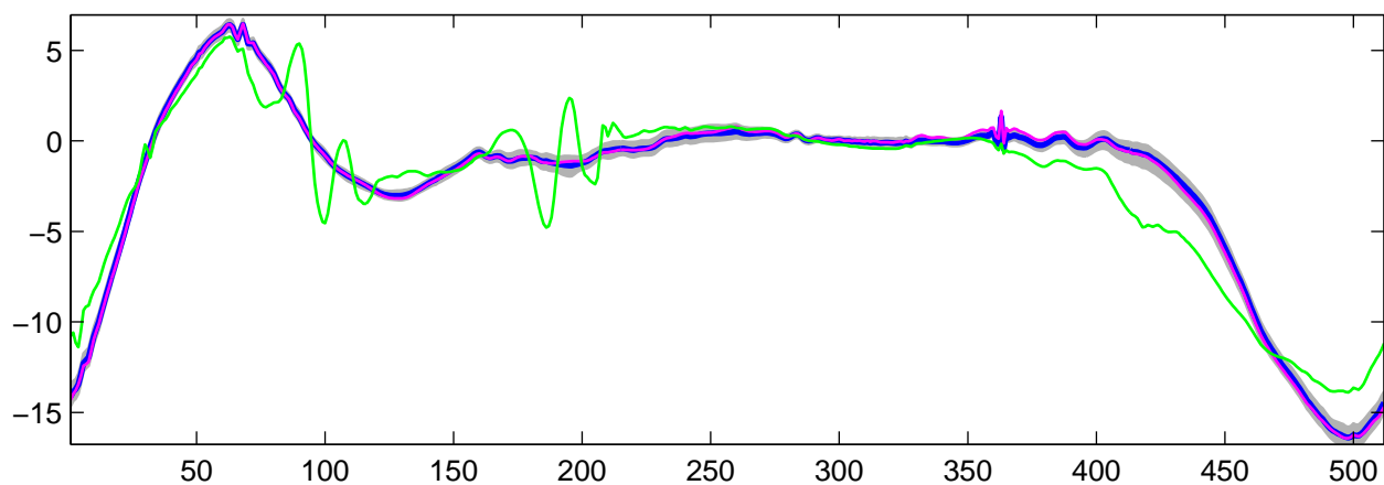
Estimated U_8(t) using R-WFMM: t_1 data, run 2
