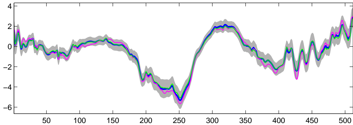
Estimated U_8(t) using G-WFMM: t_3 data, run 2
