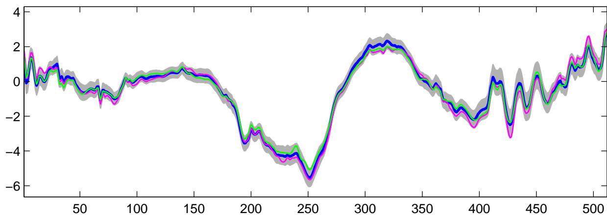
Estimated U_8(t) using R-WFMM: t_3 data, run 2
