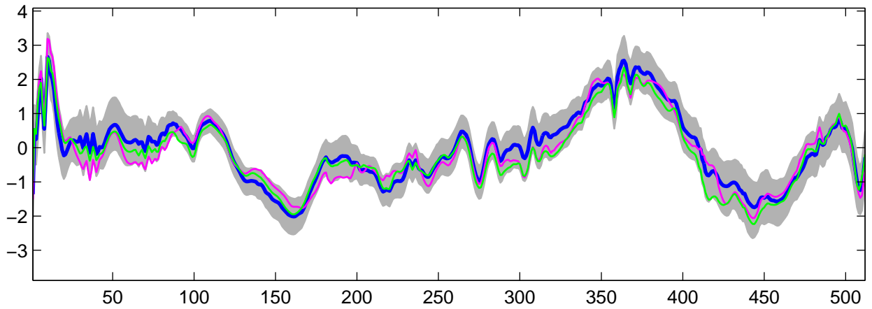
Estimated U_{\theta}(t) using R-WFMM: DE data, run 2
