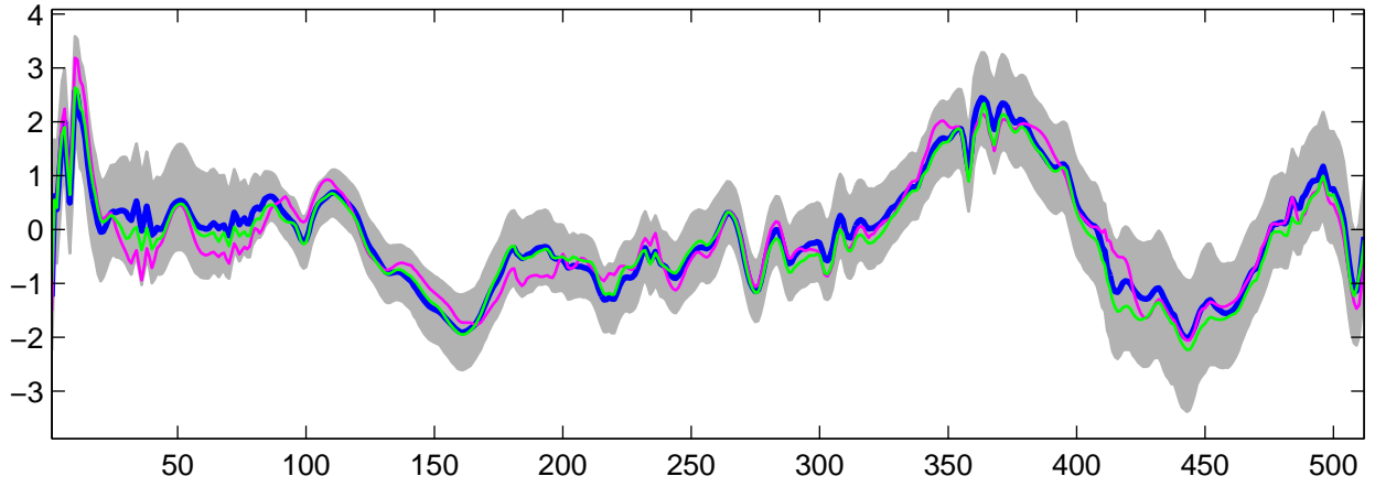
Estimated U_{\theta}(t) using G-WFMM: DE data, run 2
