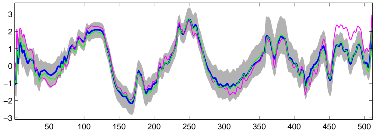
Estimated U_{\theta}(t) using R-WFMM: Normal data, run 2
