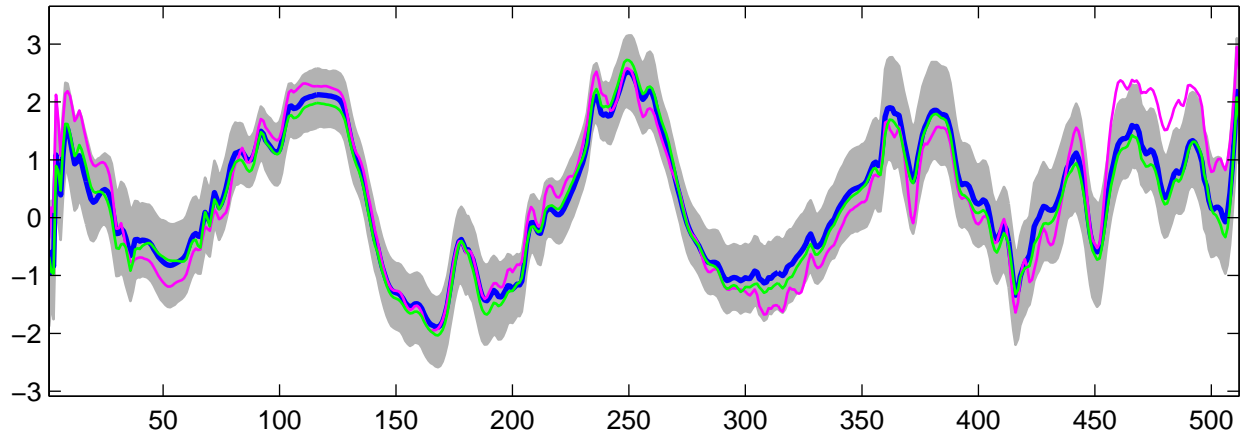
Estimated U_{\theta}(t) using G-WFMM: Normal data, run 2
