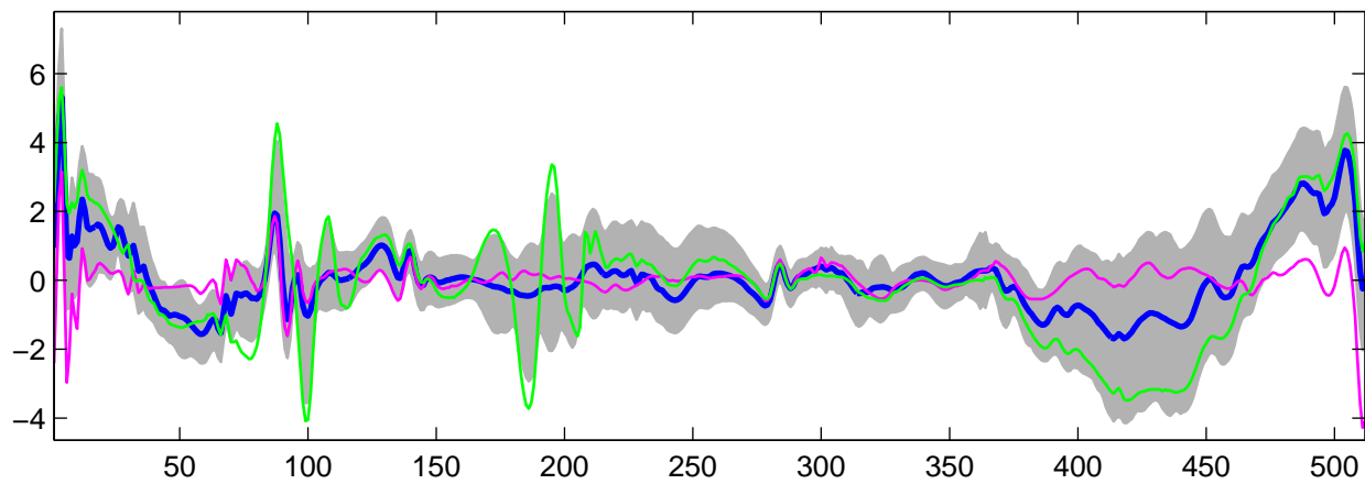
Estimated U_{\theta}(t) using G-WFMM: t_1 data, run 2
