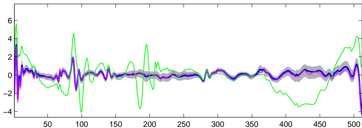
Estimated U_{\theta}(t) using R-WFMM: t_1 data, run 2
