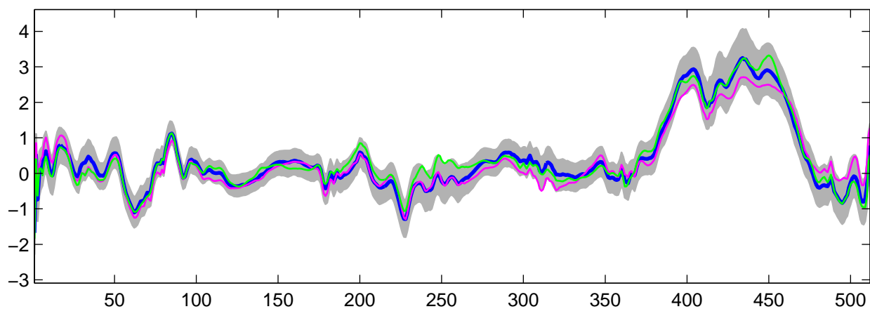
Estimated U_9(t) using R-WFMM: t_3 data, run 2
