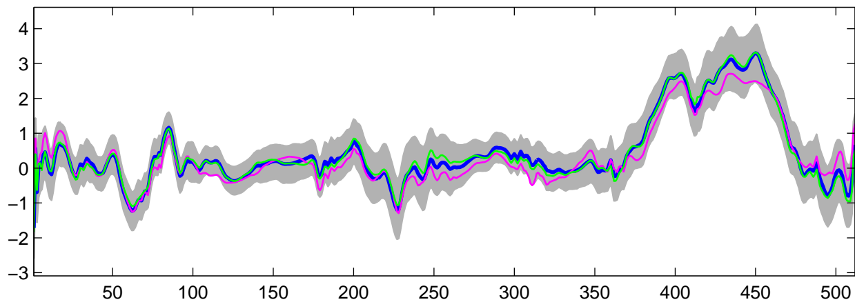
Estimated U_9(t) using G-WFMM: t_3 data, run 2
