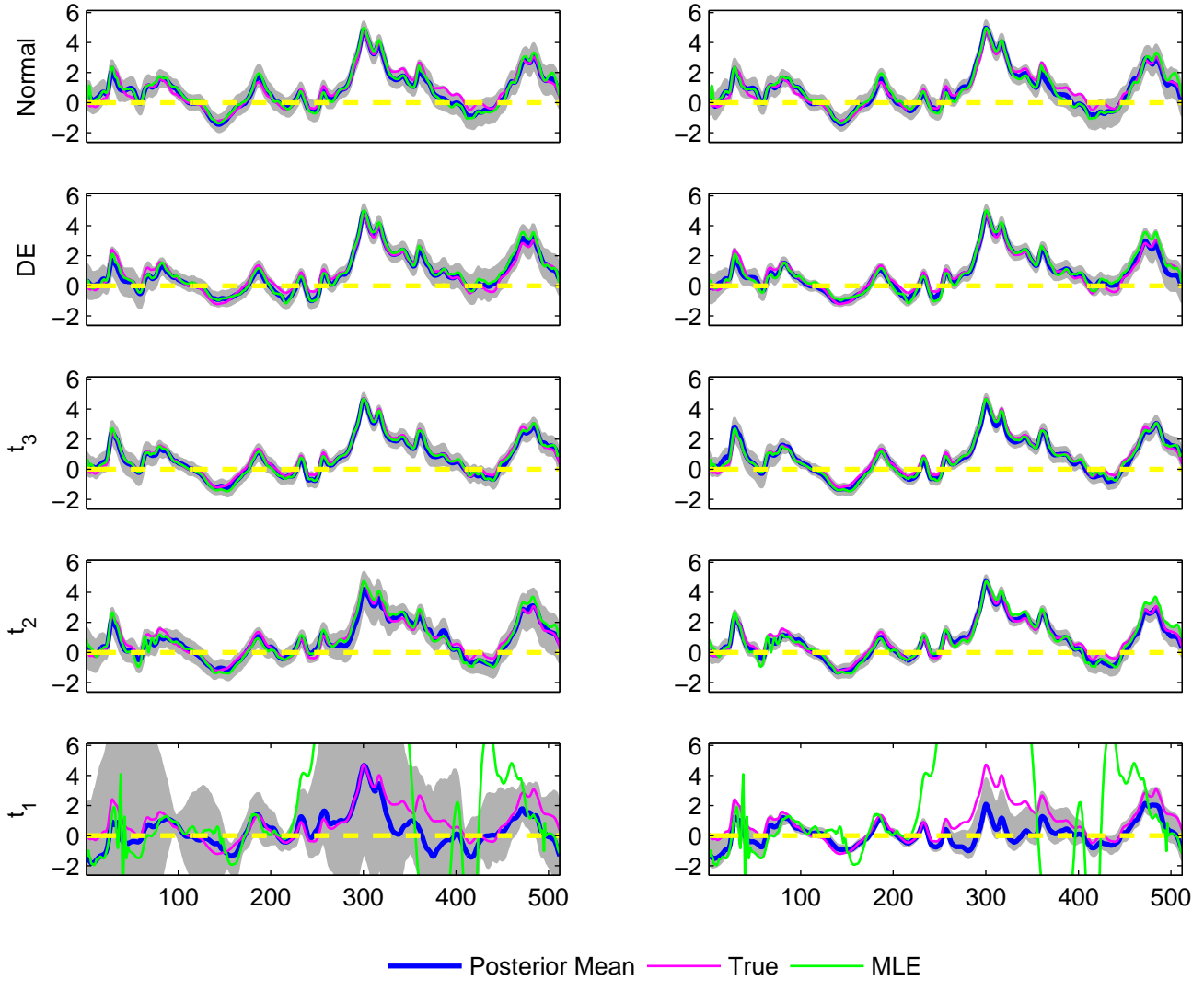
The estimated B_1(t) for 5 simulated datasets, simulation run 3 G-WFMM R-WFMM
