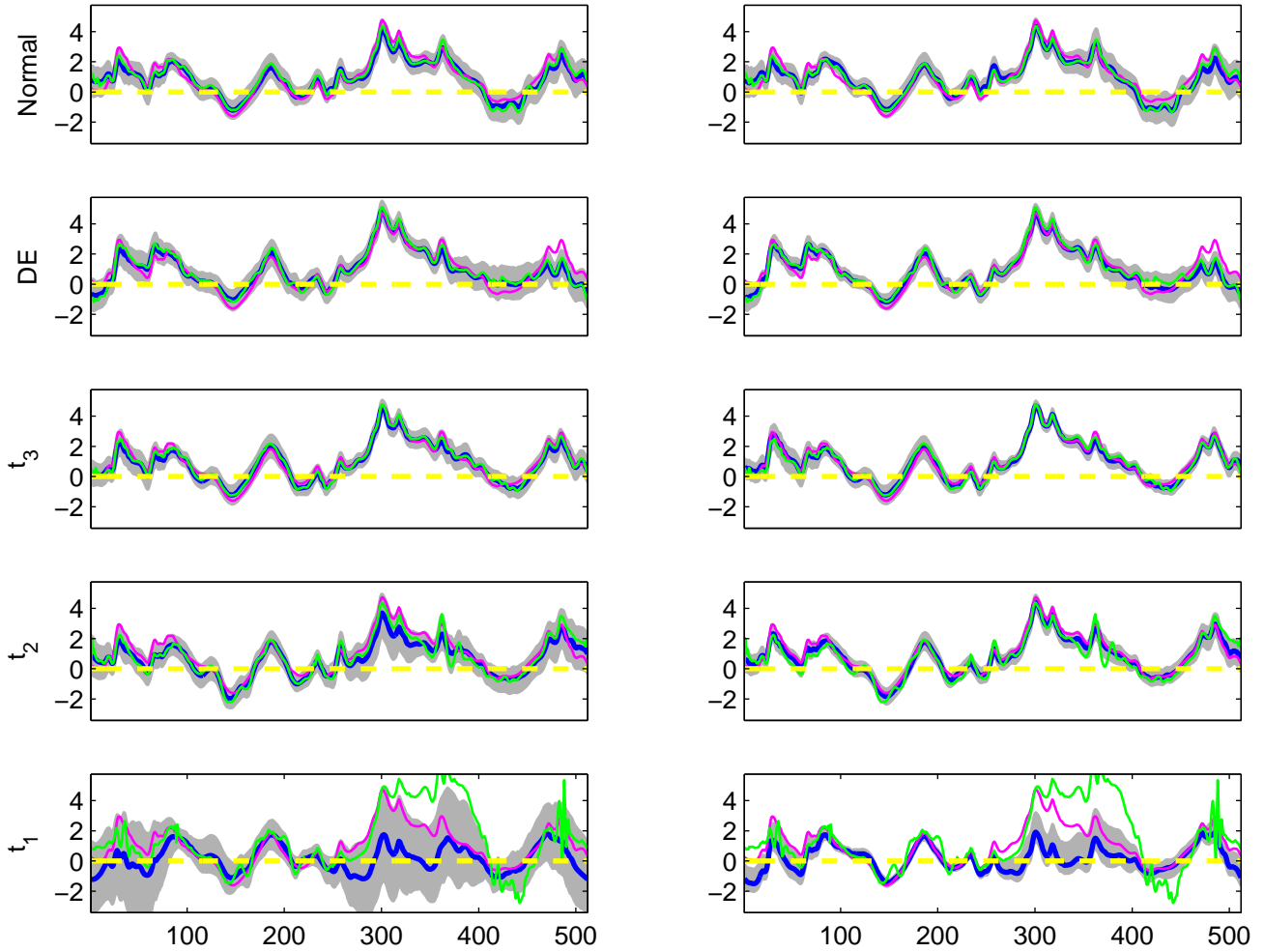
The estimated B_2(t) for 5 simulated datasets, simulation run 3 G-WFMM R-WFMM
