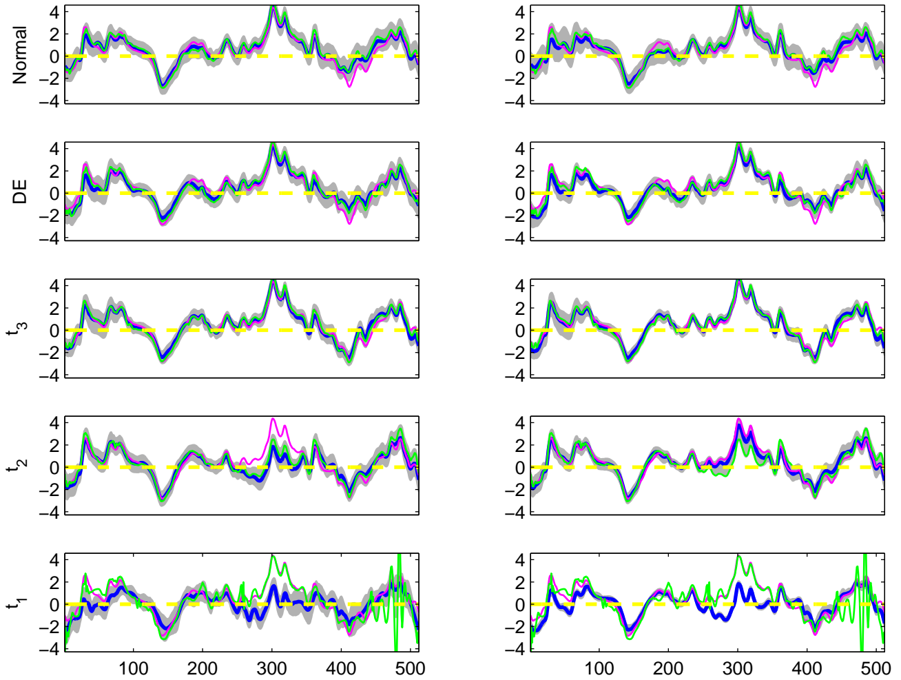
The estimated B_3(t) for 5 simulated datasets, simulation run 3 G-WFMM R-WFMM
