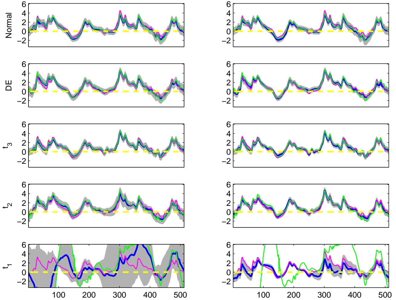
The estimated B_4(t) for 5 simulated datasets, simulation run 3 G-WFMM R-WFMM
