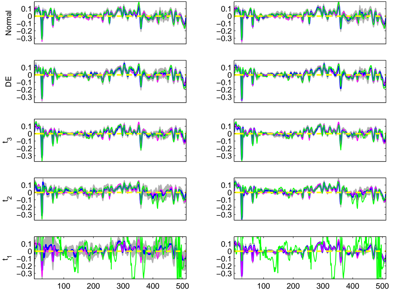
The estimated B_5(t) for 5 simulated datasets, simulation run 3 G-WFMM R-WFMM
