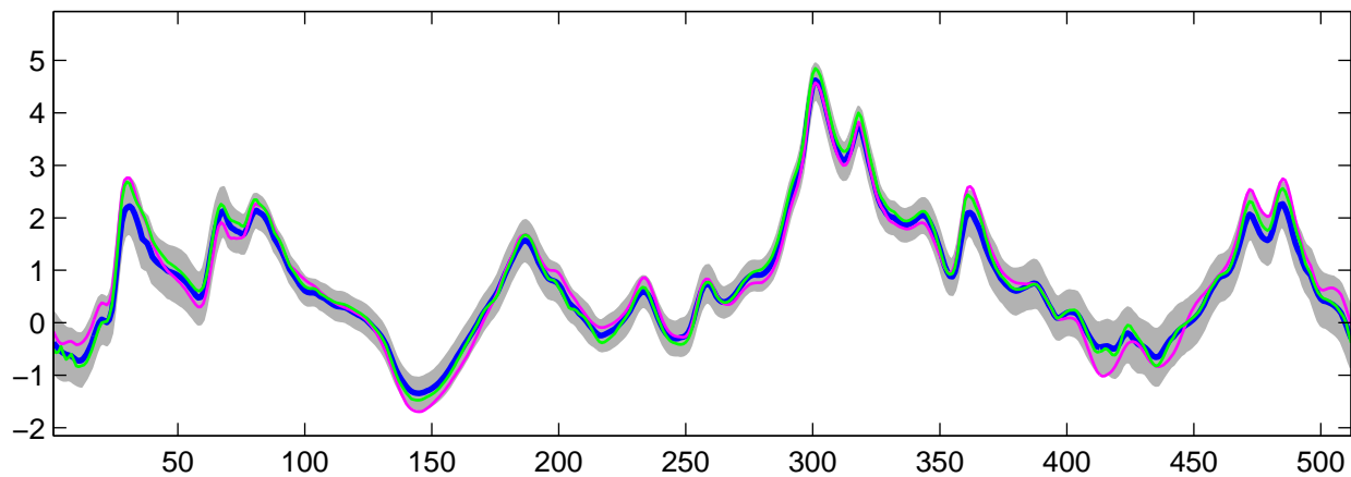
Estimated C_0(t) using G-WFMM: DE data, run 3
