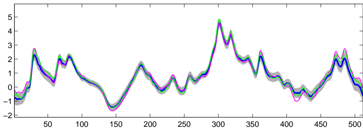
Estimated C_0(t) using R-WFMM: DE data, run 3
