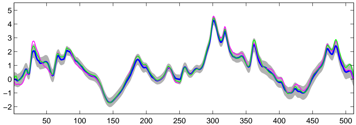
Estimated C_0(t) using R-WFMM: Normal data, run 3
