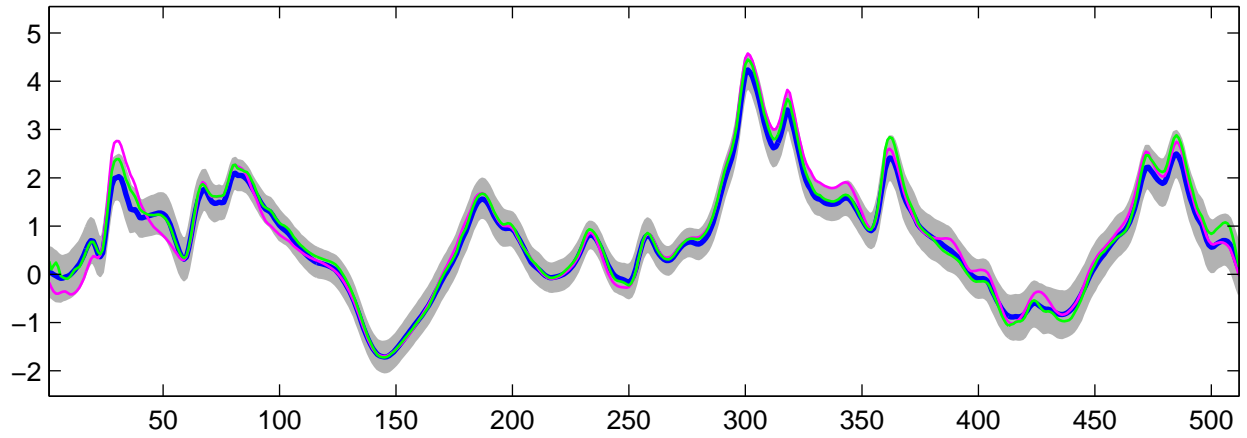
Estimated C_0(t) using G-WFMM: Normal data, run 3
