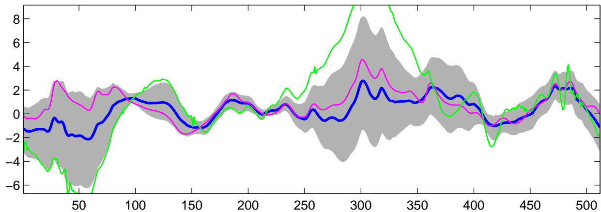
Estimated C_0(t) using G-WFMM: t_1 data, run 3
