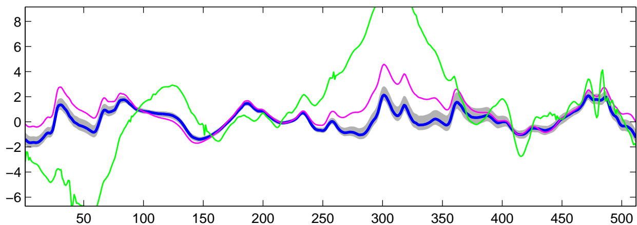
Estimated C_0(t) using R-WFMM: t_1 data, run 3
