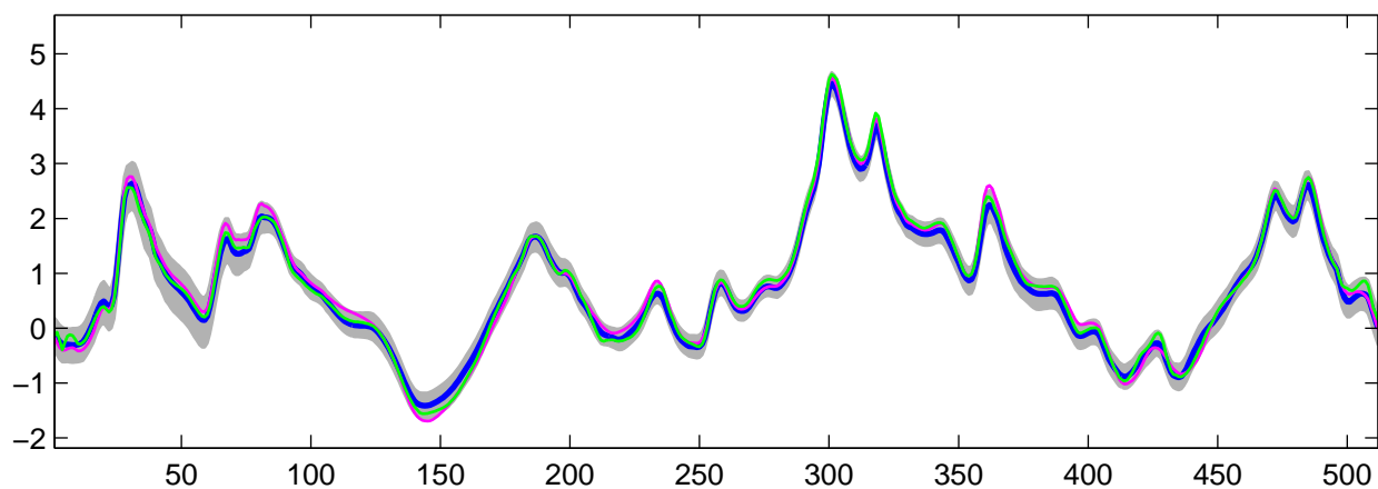
Estimated C_0(t) using R-WFMM: t_3 data, run 3
