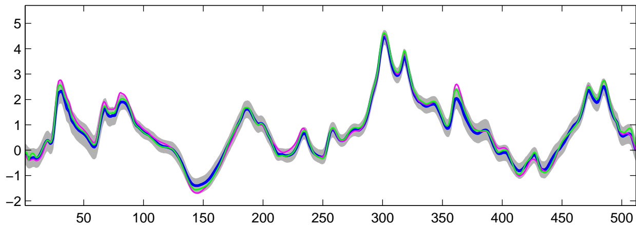
Estimated C_0(t) using G-WFMM: t_3 data, run 3
