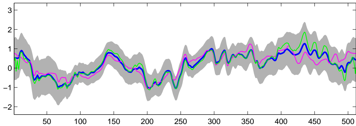
Estimated C_1(t) using G-WFMM: DE data, run 3
