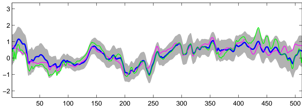
Estimated C_1(t) using R-WFMM: DE data, run 3
