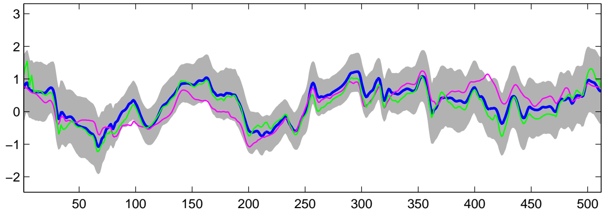
Estimated C_1(t) using R-WFMM: Normal data, run 3
