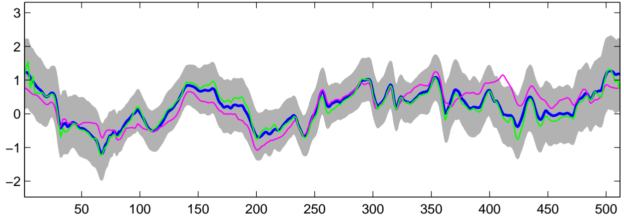
Estimated C_1(t) using G-WFMM: Normal data, run 3
