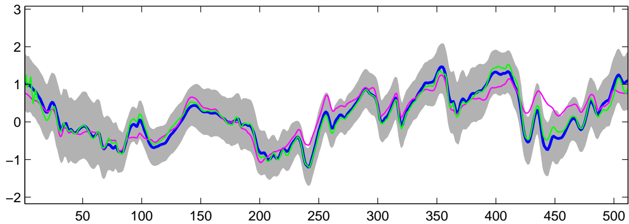
Estimated C_1(t) using G-WFMM: t_3 data, run 3
