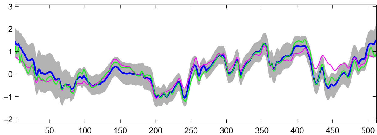
Estimated C_1(t) using R-WFMM: t_3 data, run 3
