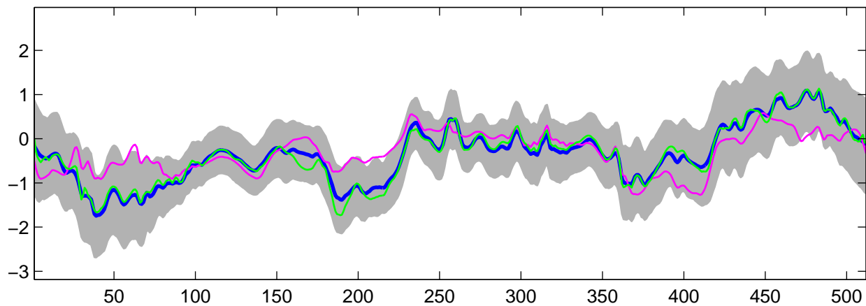
Estimated C_2(t) using G-WFMM: DE data, run 3
