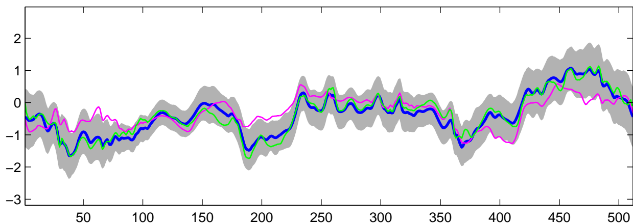
Estimated C_2(t) using R-WFMM: DE data, run 3
