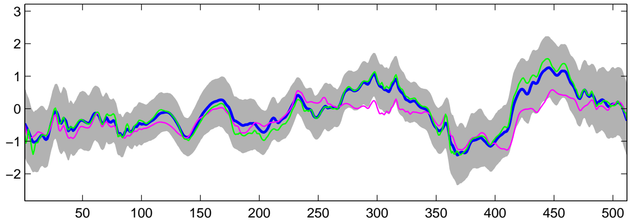
Estimated C_2(t) using G-WFMM: Normal data, run 3
