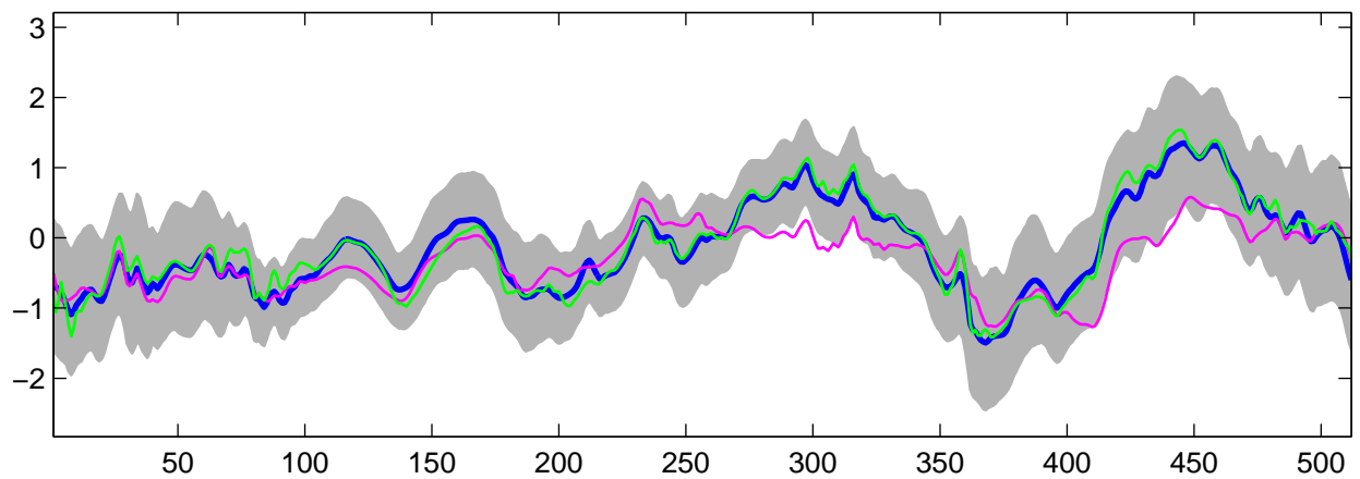
Estimated C_2(t) using R-WFMM: Normal data, run 3
